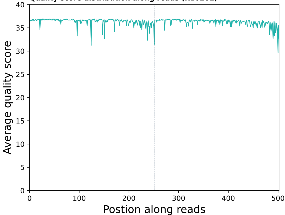
Quality score distribution along reads (R10202)
